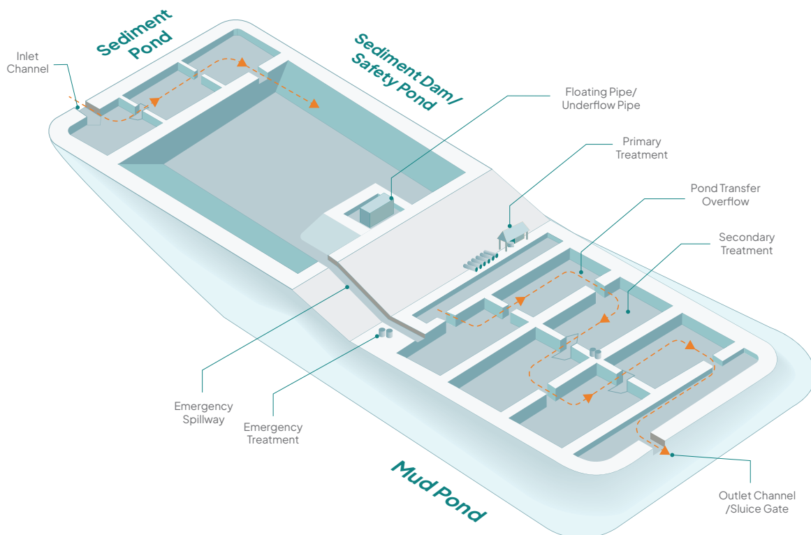
Mine waste water treatment process at AMI (settling ponds) Proses pengelolaan air limbah tambang di AMI (settling ponds)
